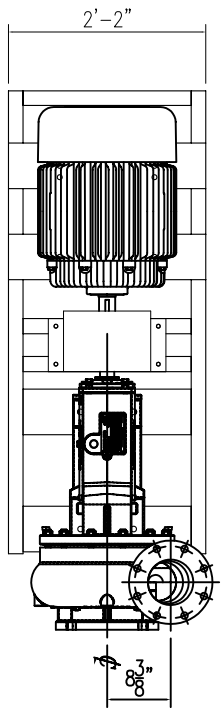
PLAN VIEW 1 1/2" = 1'-0"
