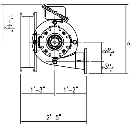
END VIEW 1 1/2" = 1'-0"
