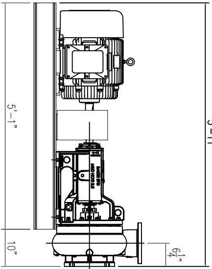
ELEVATION 1 1/2" = 1'-0"
