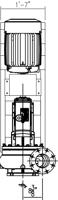
PLAN VIEW 1 1/2" = 1'-0"
